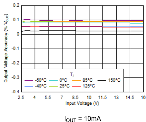
Figure 5-3. V_{OUT} Accuracy vs V_{IN} (Fixed Output, New Chip)
