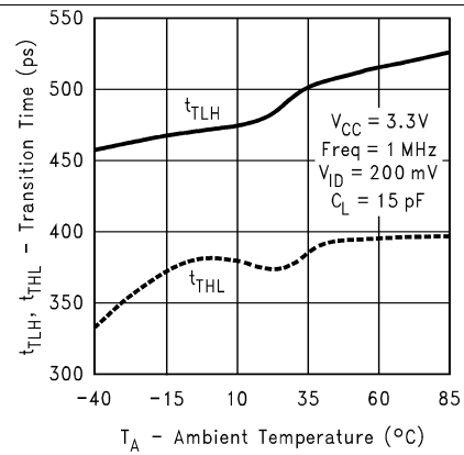
Figure 15. Transition Time vs Ambient Temperature
