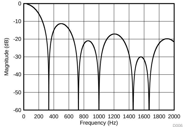
Figure 50. Filter Response (Normal Mode, DR = 330 SPS)
