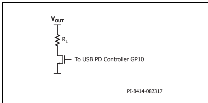
Figure 13. Active Pre-Load Circuit.
