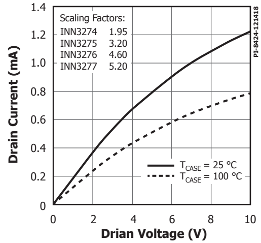
Figure 32. Output Characteristics.
