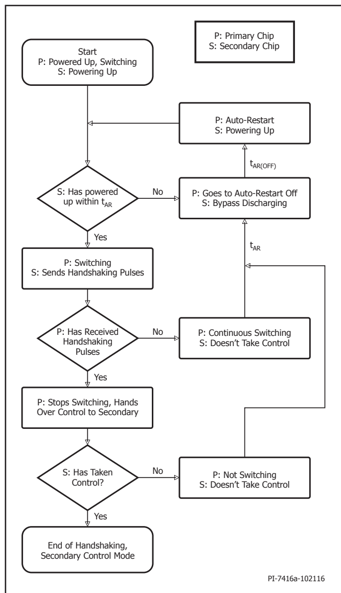
Figure 8. Primary-Secondary Handshake Flowchart.
