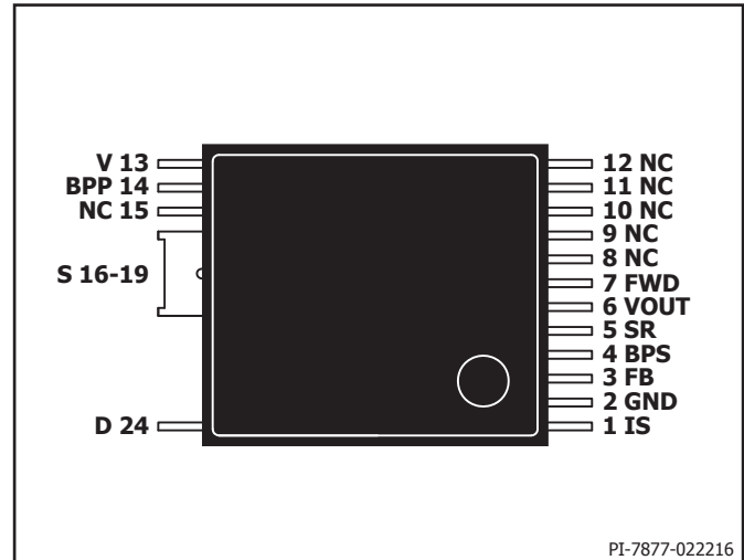
Figure 6. Pin Configuration.
