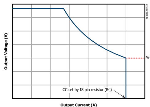
Figure 3. Typical Constant Power Characteristics.
