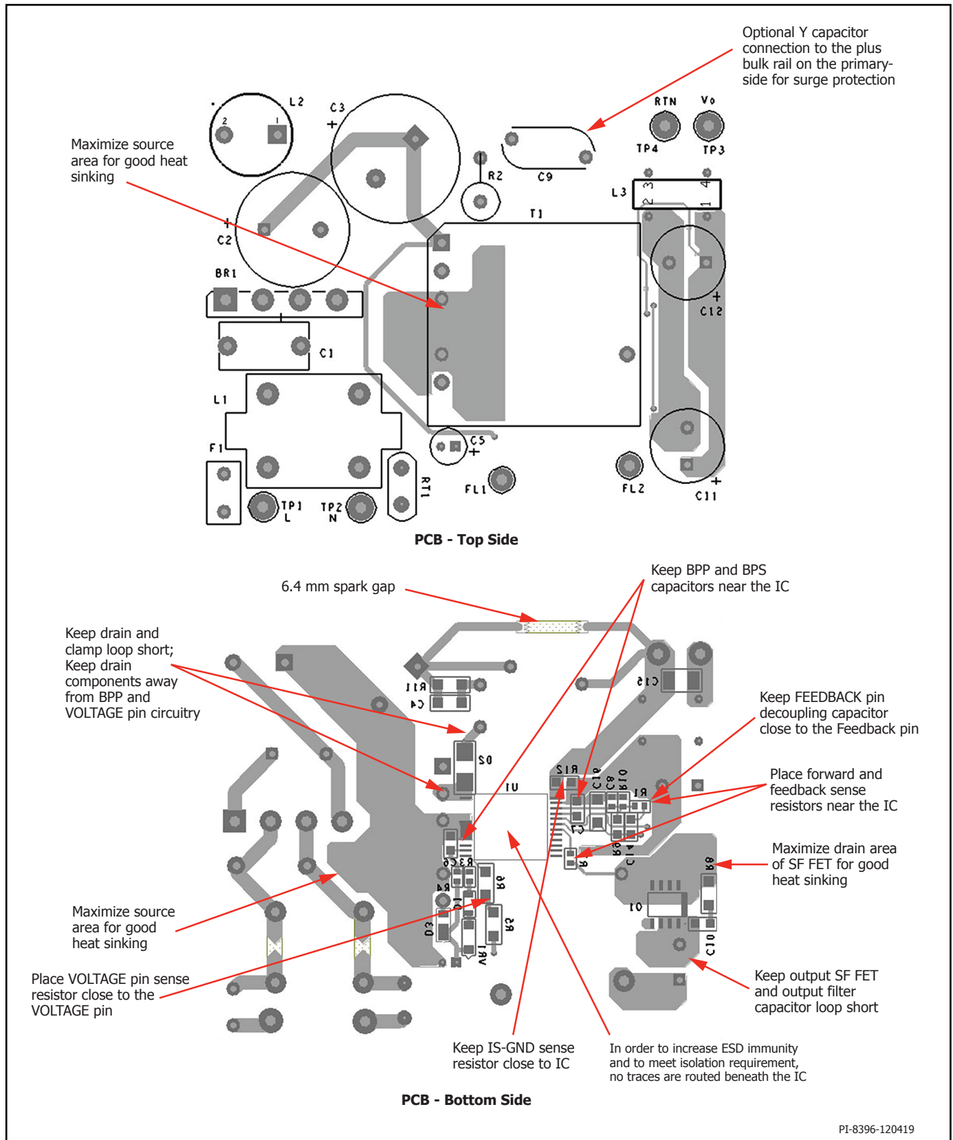
Figure 20. PCB.
