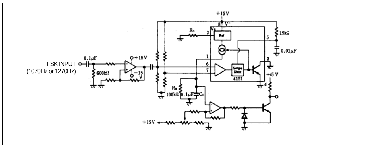
Figure 8. FSK demodulator
