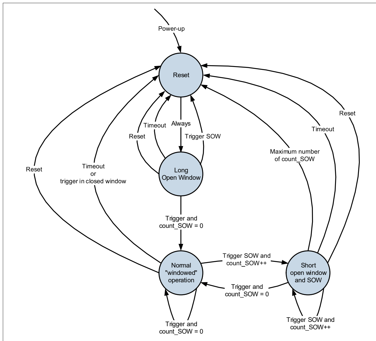
Figure 14 Watchdog timer behavior
