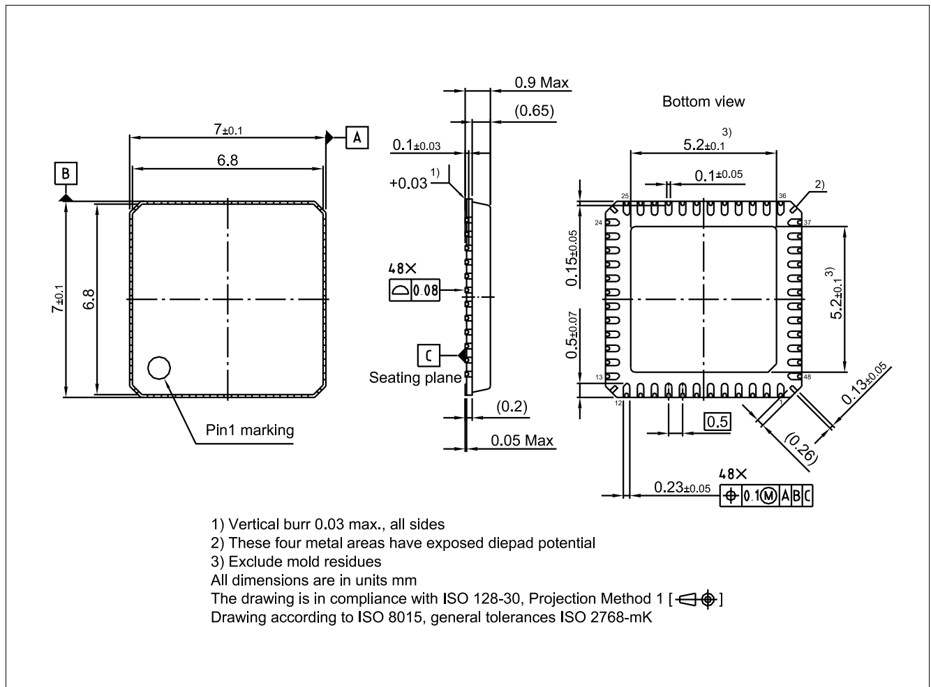
Figure 37 Package outline VQFN-48-37 with LTI (UH and UI step) 1)
