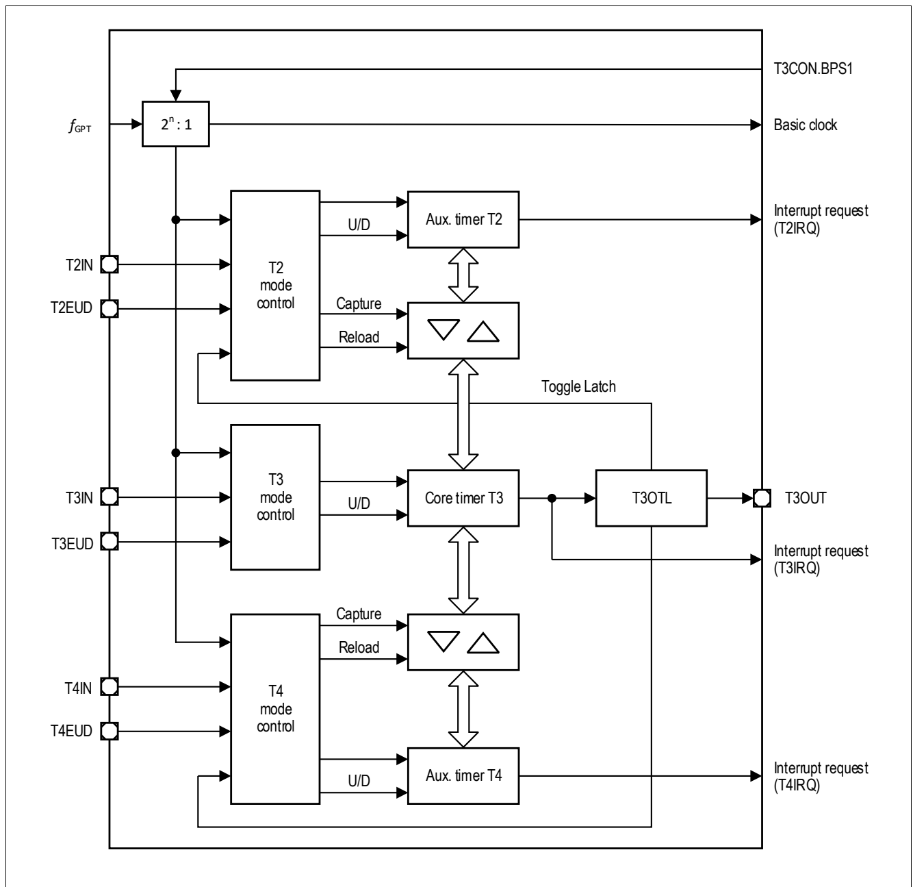
Figure 17 GPT1 block diagram ( n = 2 \dots 5 )
