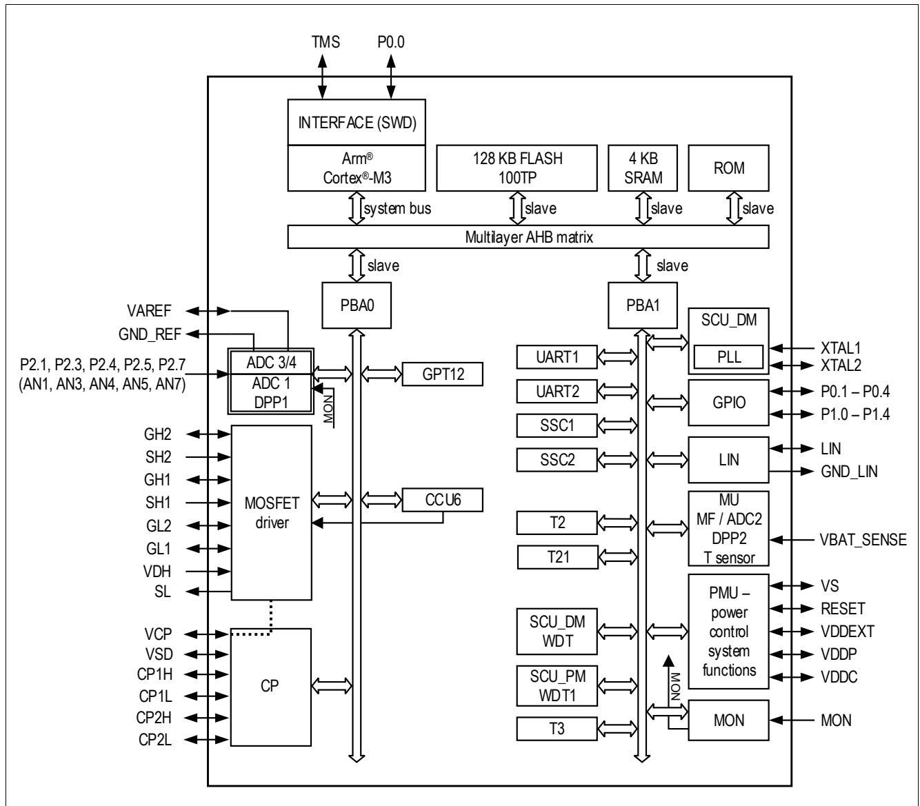
Figure 1 Block diagram
