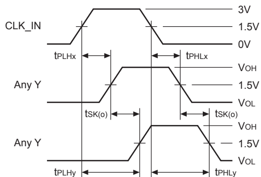
Output Skew – t_{sk(o)}
