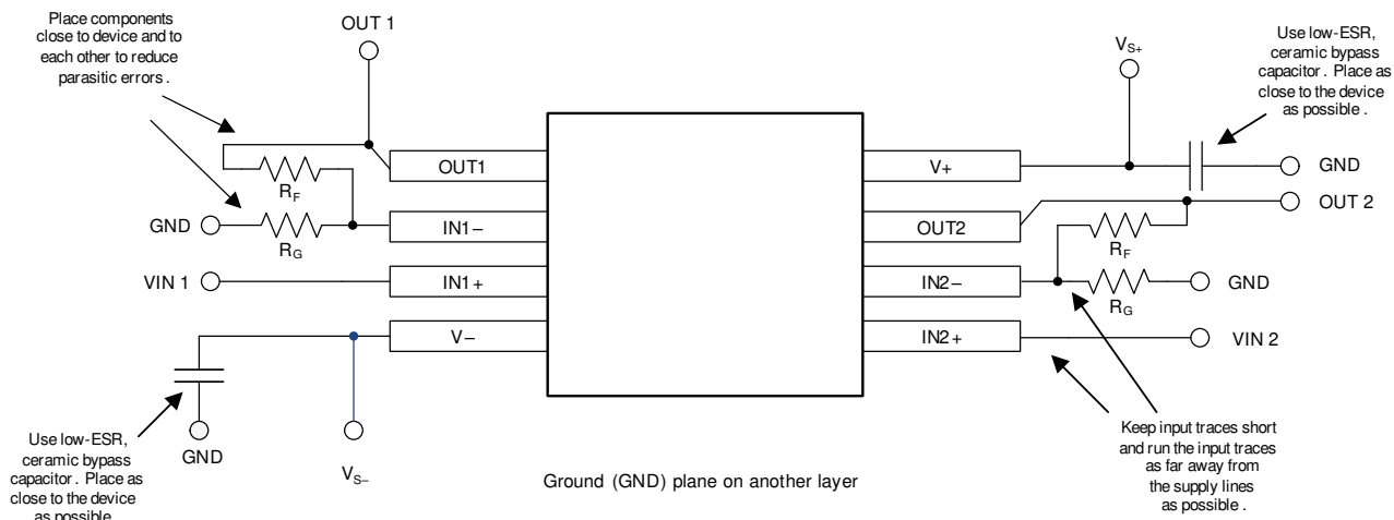
Figure 8-5. Layout Example
