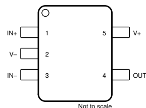
Figure 5-2. TLV9061 DCK Package, 5-Pin SC70 (Top View)
