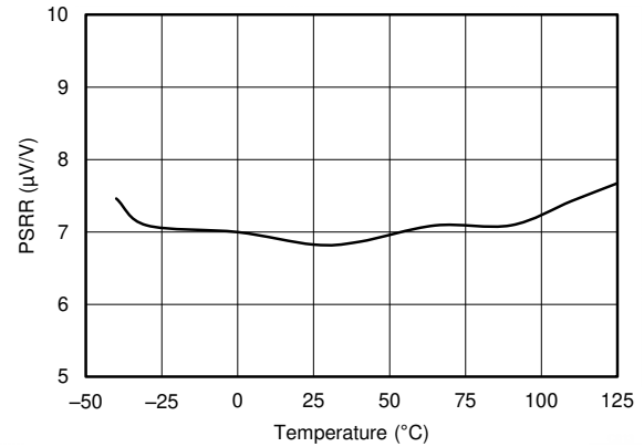
Figure 6-14. PSRR vs Temperature
