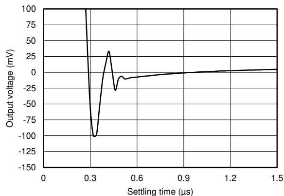
Figure 6-36. Large Signal Settling Time (Negative)
