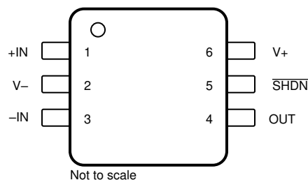
Figure 5-5. TLV9061S DRY Package, 6-Pin USON (Top View)
