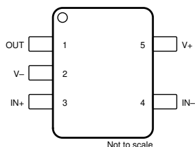
Figure 5-1. TLV9061 DBV or DRL Package, 5-Pin SOT-23 or SOT-553 (Top View)
