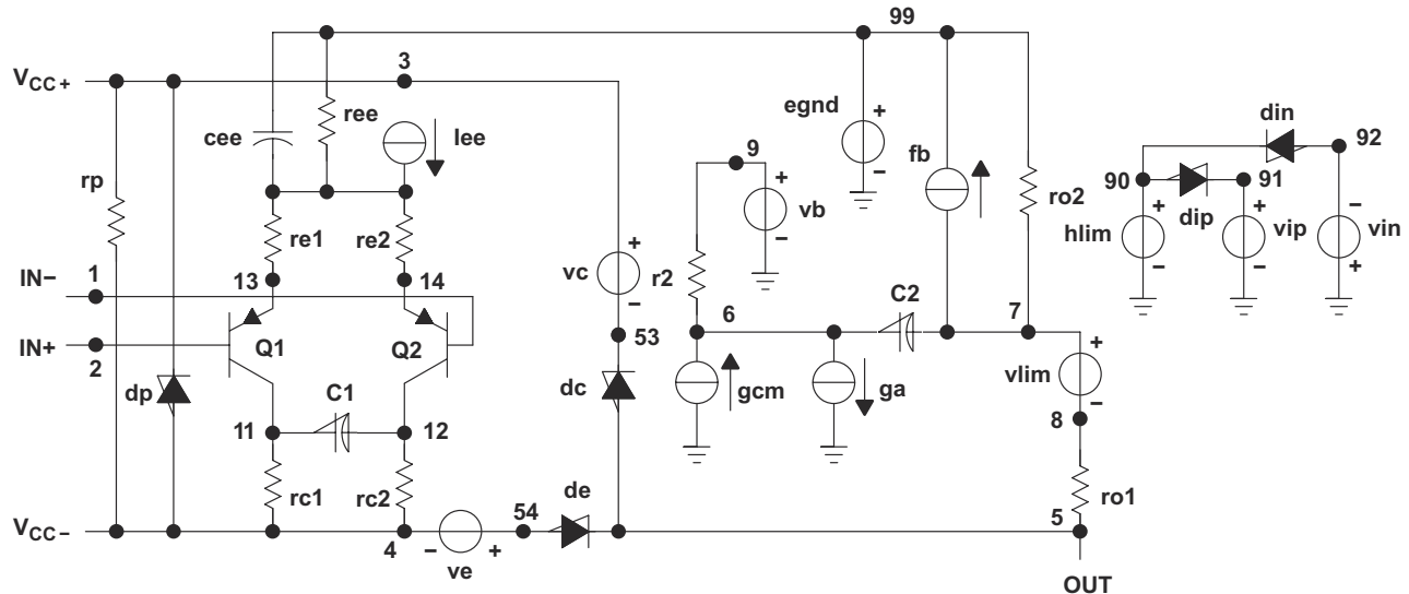
Figure 8-3. Boyle Subcircuit
