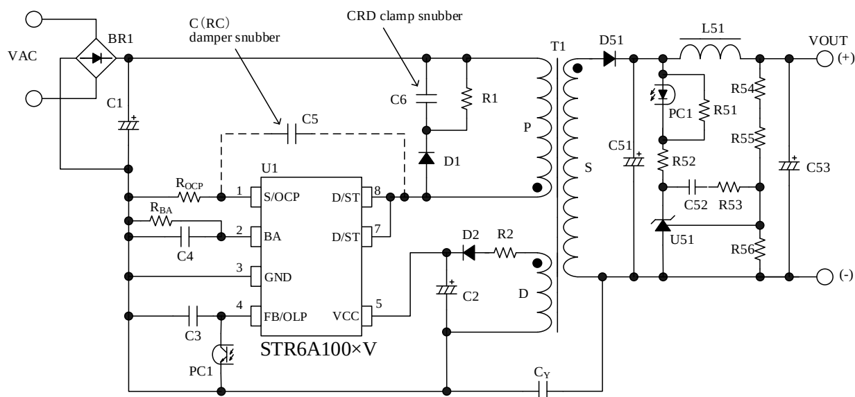
Figure 6-1. Typical Application
