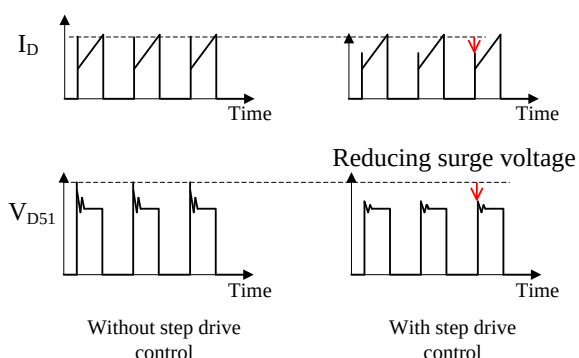
Figure 9-10. I_D and V_{D51} Waveforms
