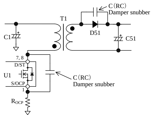
Figure 9-15. Damper Snubber
