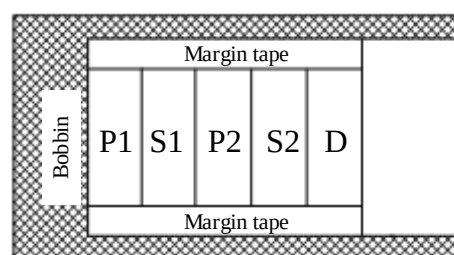
Winding Structural Example (a)
