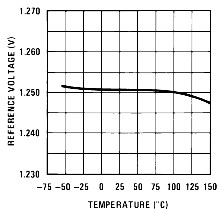
Figure 5-5. Temperature Stability
