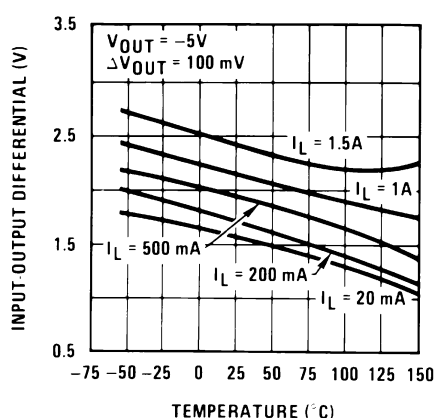
Figure 5-4. Dropout Voltage
