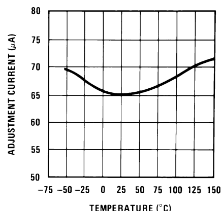
Figure 5-3. Adjustment Current
