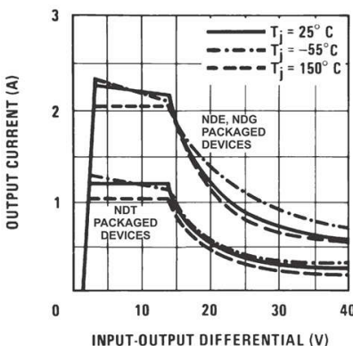
Figure 7-2. Current Limit
