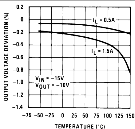
Figure 5-1. Load Regulation
