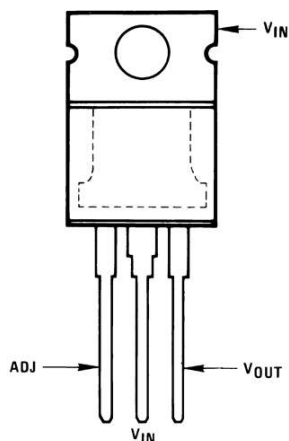
Figure 4-1. TO-220 Plastic Package Package Number NDE0003B Front View
