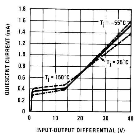
Figure 5-6. Minimum Operating Current
