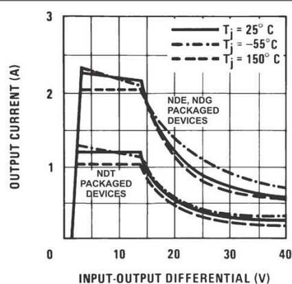
Figure 5-2. Current Limit
