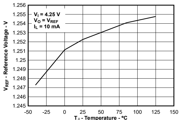
Figure 5-8. V_{REF} Temperature Stability vs Temperature (New Chip)
