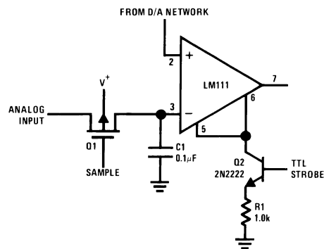
Figure 30. Relay Driver with Strobe
