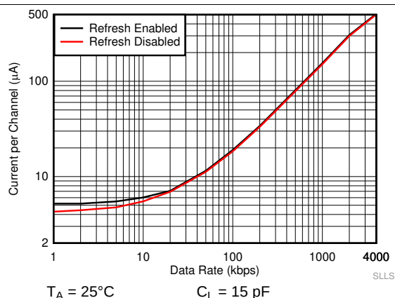
Figure 10. ISO7041 Supply Current vs Data Rate at 5 V (With 15-pF Load)
