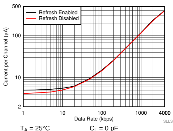
Figure 9. ISO7041 Supply Current vs Data Rate at 5 V (With No Load)
