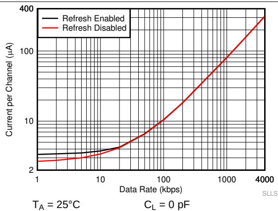
Figure 3. ISO7041 Supply Current vs Data Rate at 1.8 V (With No Load)
