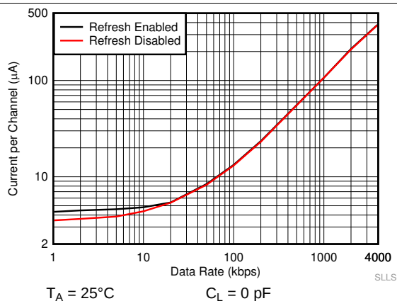
Figure 7. ISO7041 Supply Current vs Data Rate at 3.3 V (With No Load)
