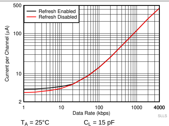
Figure 6. ISO7041 Supply Current vs Data Rate at 2.5 V (With 15-pF Load)
