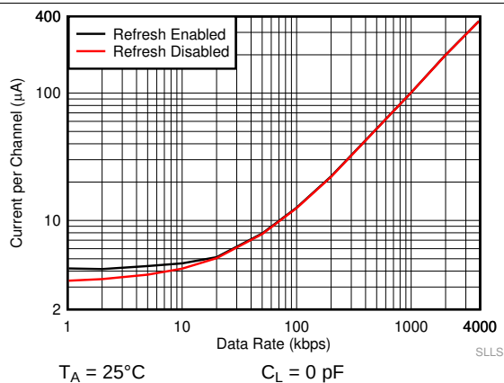
Figure 5. ISO7041 Supply Current vs Data Rate at 2.5 V (With No Load)
