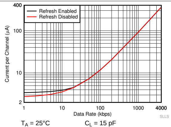
Figure 4. ISO7041 Supply Current vs Data Rate at 1.8 V (With 15-pF Load)
