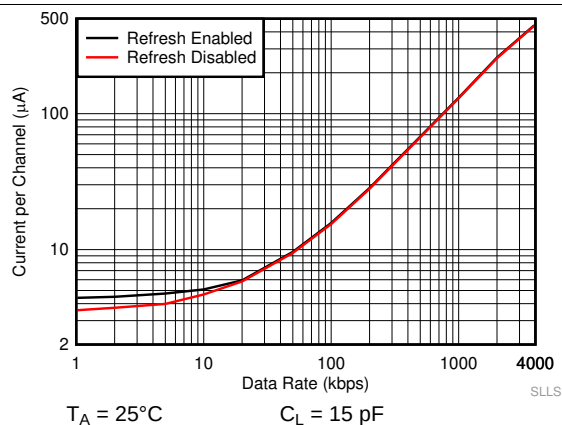
Figure 8. ISO7041 Supply Current vs Data Rate at 3.3 V (With 15-pF Load)
