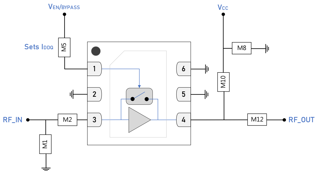
GRF2374 Standard Evaluation Board Schematic
