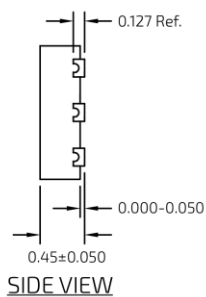
DFN-6 1.5 x 1.5 mm DFN-6 Package Dimensions
