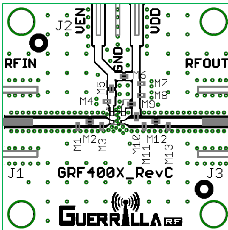
GRF2374 Evaluation Board Assembly Diagram
