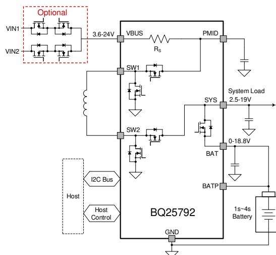
Simplified Schematic
