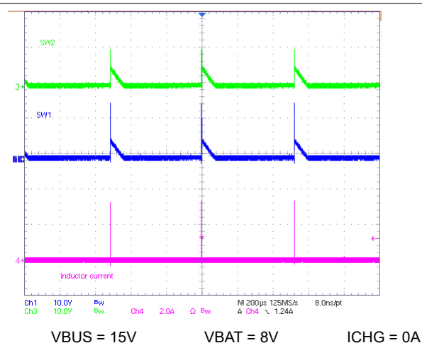
Figure 10-4. Buck Mode PFM without OOA
