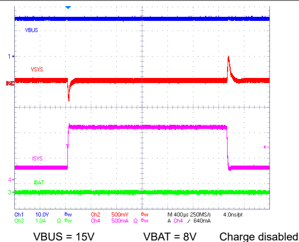
Figure 10-7. VSYS Load Transient Response
