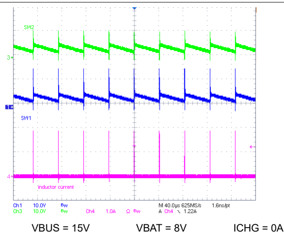
Figure 10-3. Buck Mode PFM with OOA
