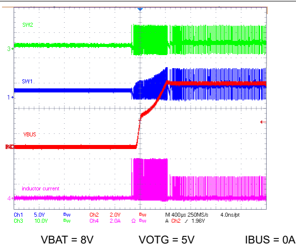
Figure 10-5. OTG Startup at No Load
